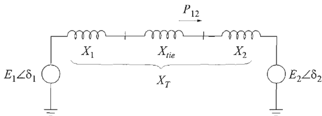
Figure 1 Two area system
