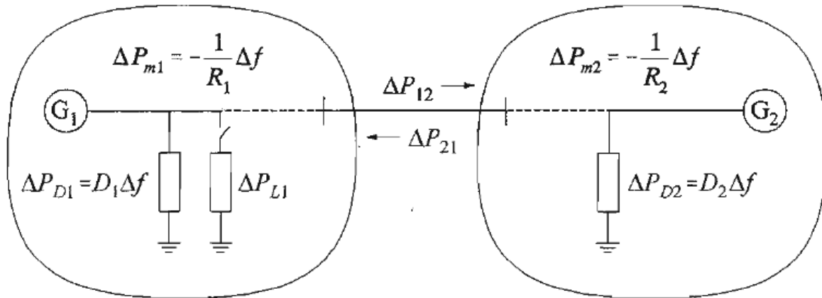
Figure 5 Effect of change in area 1 load
