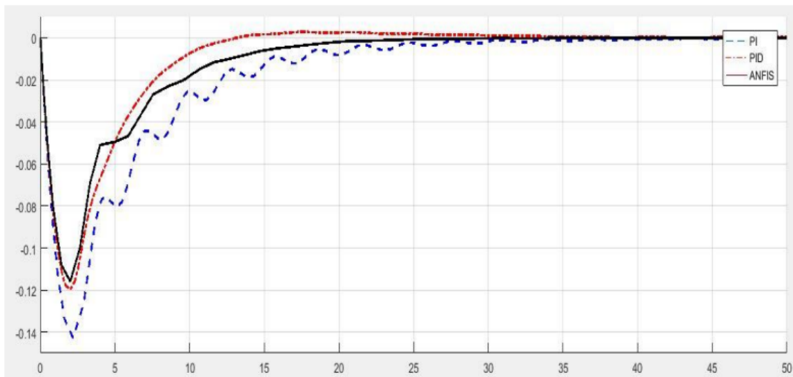
Figure 7 Frequency deviation of area 1
