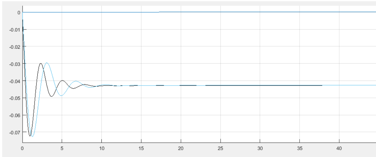
Figure 4 Steady state frequency deviation for two area system due to primary control
