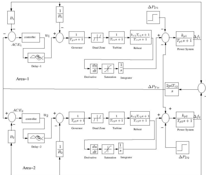
Figure 6 Two area power system considering generation rate constraint and governor dead-band [4] [15]
