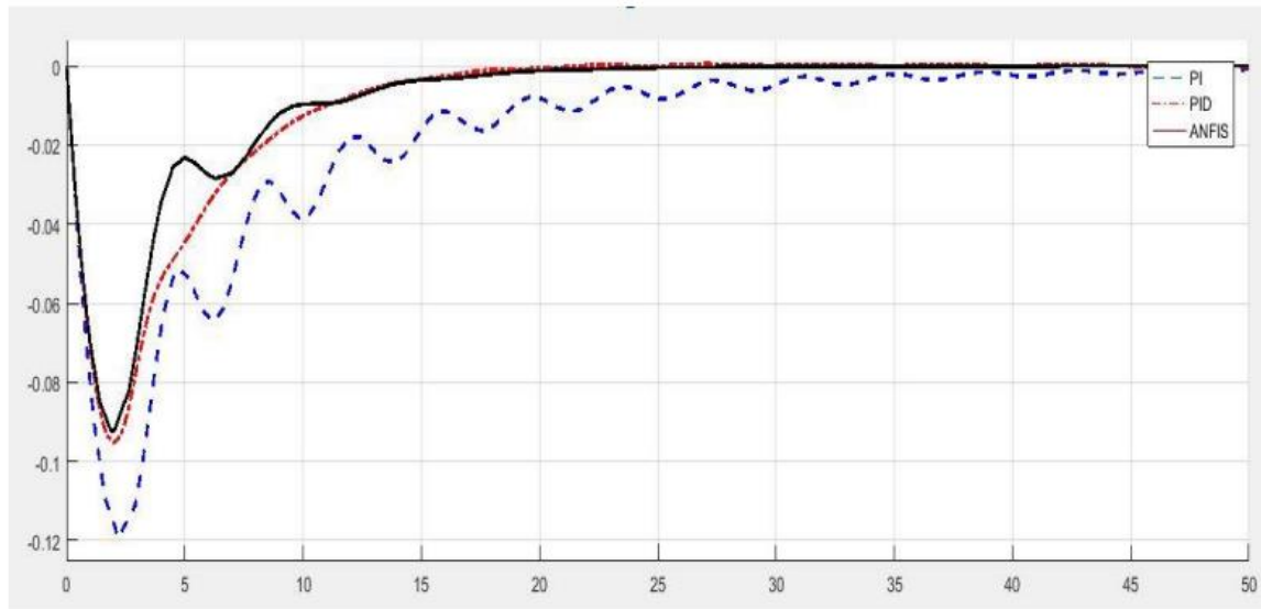
Figure 8 Frequency deviation of area 2
