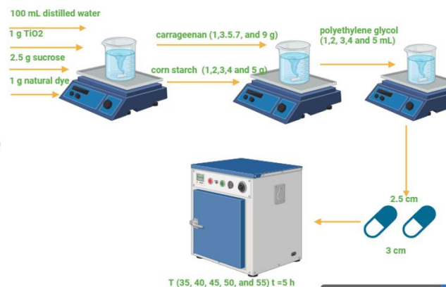
Fig The making Capsule Shell Steps
