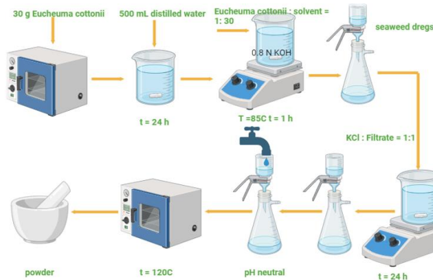
Fig The making carrageenan steps
