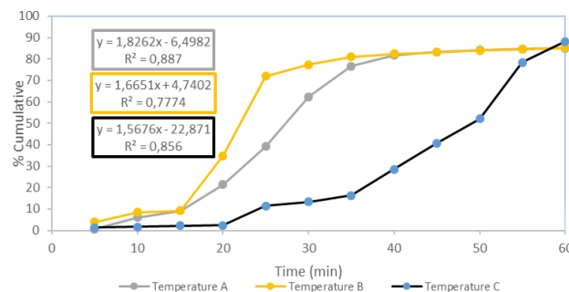
Figure 8. Dissolution test temperature variations
