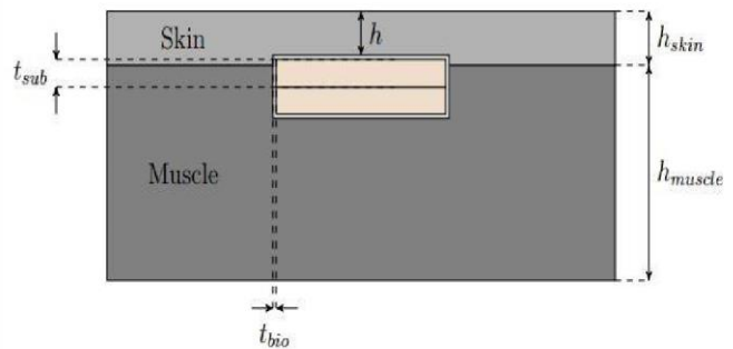
(b) Antenna inside the two-layer geometry model
