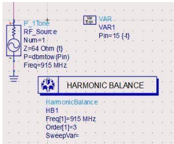
(a) HB simulator setup for single tone
