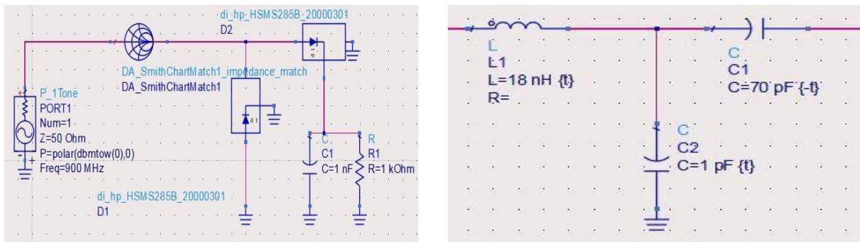
Figure 3. Rectenna design along with RF signal generation
