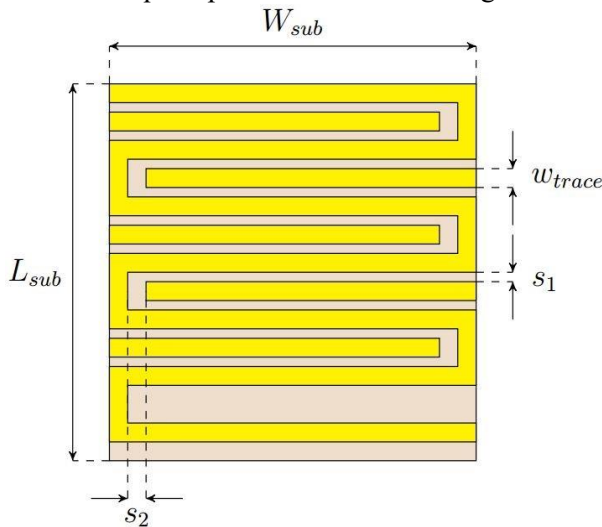
(a) Patch with all the dimensional parameters of the antenna
