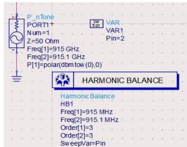
(b) HB simulator setup for dual tone
