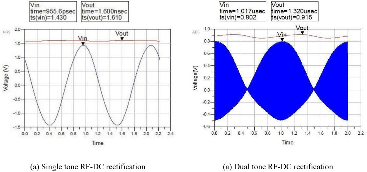
Figure 7. Double stage RF-DC conversion
