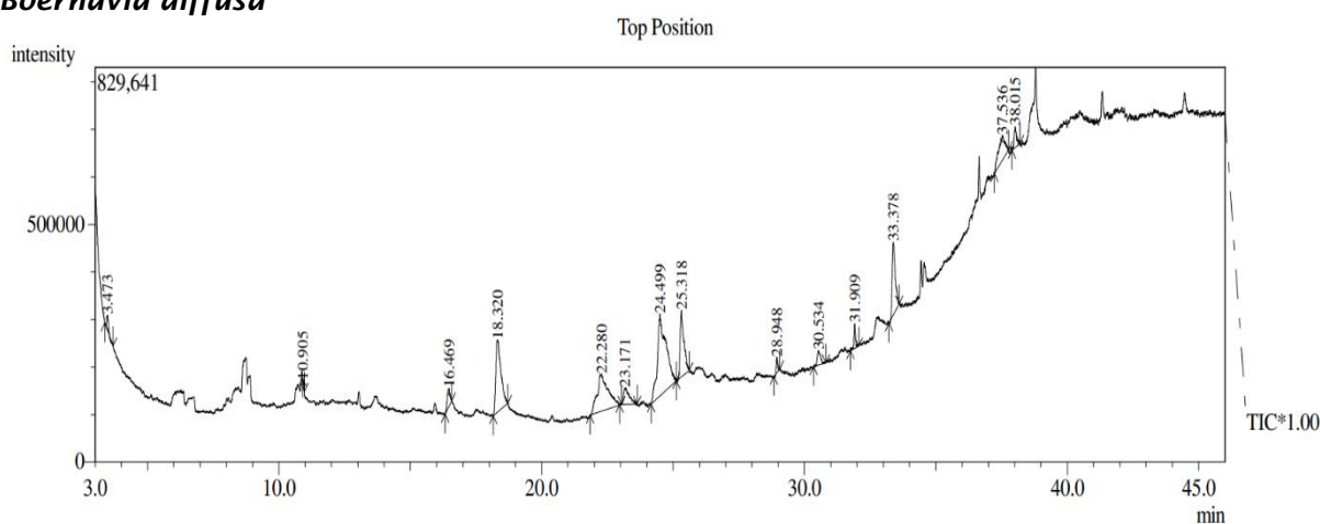
Fig VI: GC-MS/MS chromatogram of ethanolic extract of roots of Boerhavia diffusa
