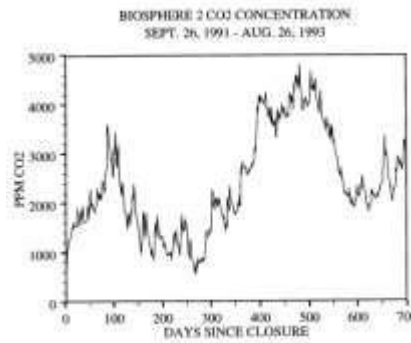
Fig 3.4: [7] Carbon Dioxide levels in Biosphere 2
