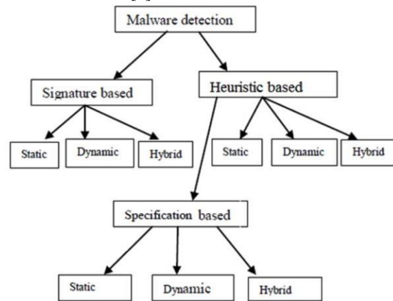
Fig 2: Types of Malware Detection
