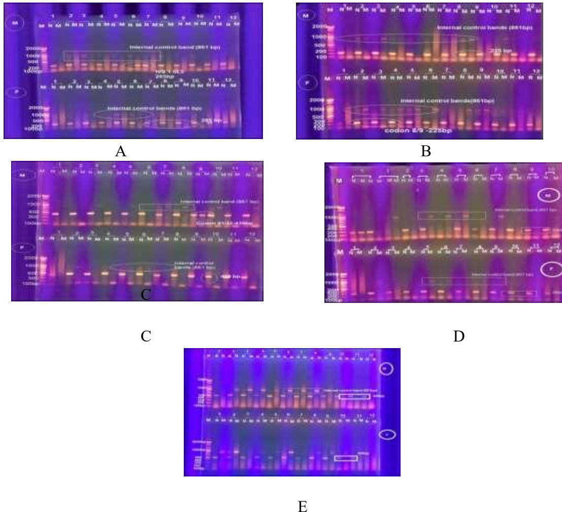
Figure (1) ARMS-PCR products on 2% agarose gel electrophoresis at 60 voltages for 45 min. A-IVS-1-5(G-C) mutation (285 bp); B-Codon 8/9 (+G) mutation (225 bp); C-Codon 41/42 (TCTT) mutation (439 bp); D-Codon 30 (G-C) mutation (280 bp); E-Codon 8 (+AA) mutation (255 bp); Marker: ladder marker (100 bp) DNA; N: normal; M: mutant.
