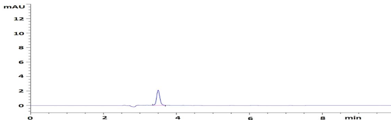
Fig. 4. Chromatogram of standard solution (LOQ concentration)
