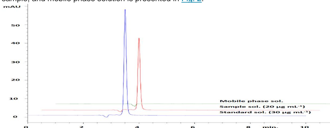
Fig. 2. Chromatogram of standard ( 30 \mu\text{g mL}^{-1} ), sample ( 20 \mu\text{g mL}^{-1} ), and mobile phase solution
