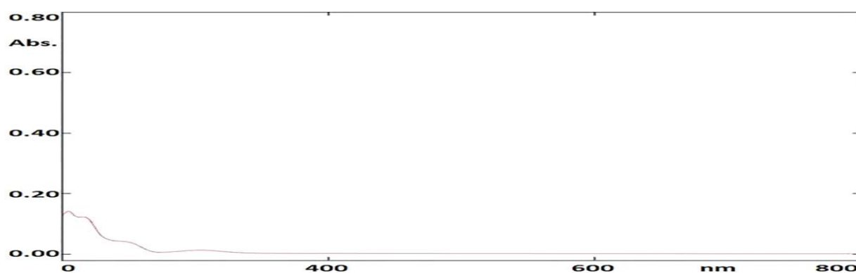
Fig. 5. Spectrum of sample solution (LOQ concentration)
