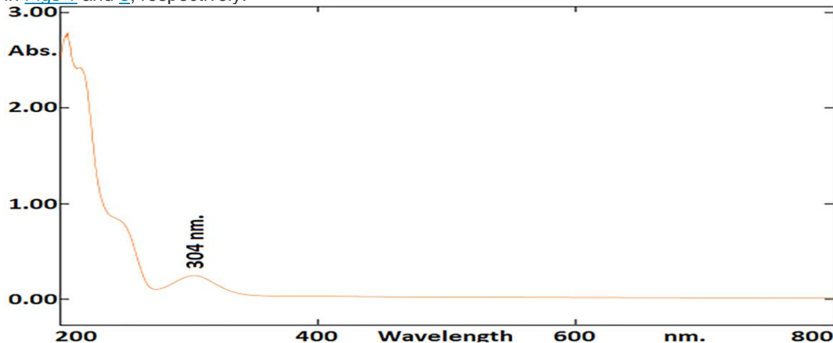
Fig. 3. Spectrum of sample solution ( 20 \mu\text{g mL}^{-1} )
