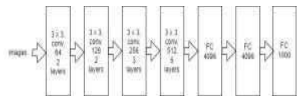
Figure 2. VGG-16 model
