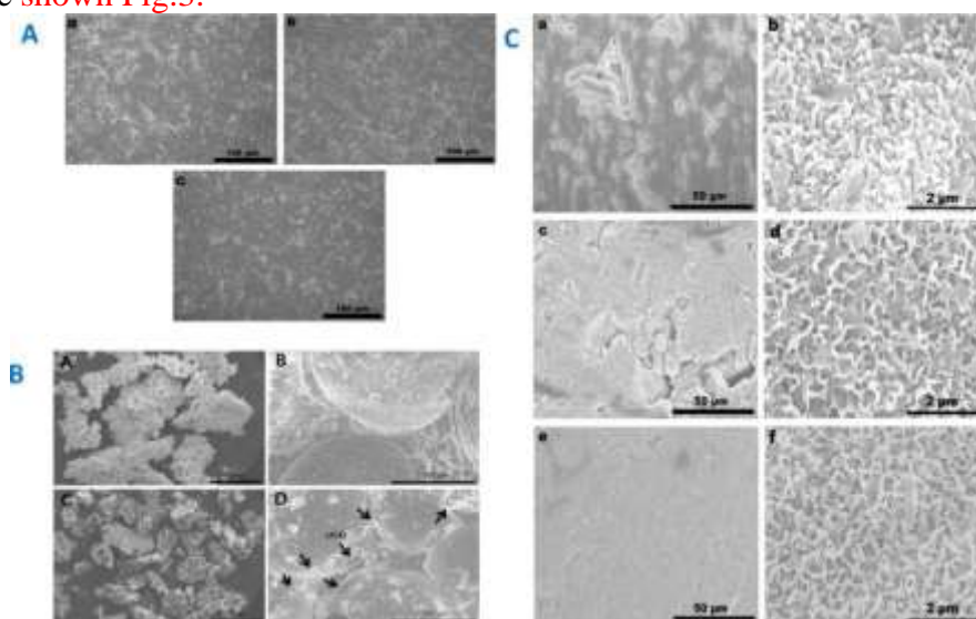
Figure 3. A) SEM images of the surfaces of (a) HA, (b) 0.5 wt.% GNS/HA composite and (c) 1.0 wt.% GNS/HA composite. Reproduced with the permission of Elsevier copyright@2013.Ref.129. B) Field emission scanning electron microscope (FE-SEM) images of biphasic calcium phosphate (BCP) microparticles (magnification: 30x (A); 500x (B)) and reduced graphene oxide (rGO)-coated BCP bone graft materials (magnification: 30 x(C); 500x(D)). Arrows indicate the rGO nanoplatelets. Ref.9. C) Low- and high-magnification SEM images of apatite formation on HA (a and b), 0.5 wt.% GNS/HA composite (c and d) and 1.0 wt.% GNS/HA composite (e and f) immersed in SBF for 7 days, Reproduced with the permission of Elsevier copyright@2013.Ref.129.
