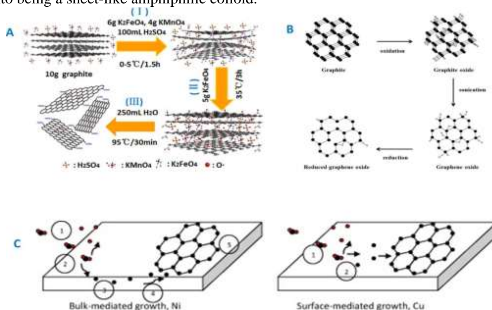
Figure 2. A) Illustration of the preparation of GO based on an newly improved Hummers method. Ref.103 B) 11. Schematic images of the process used to produce reduced graphene oxide (rGO). Ref.9. C) Reproduced with permission of Elsevier copyright @2014. Ref 104.
