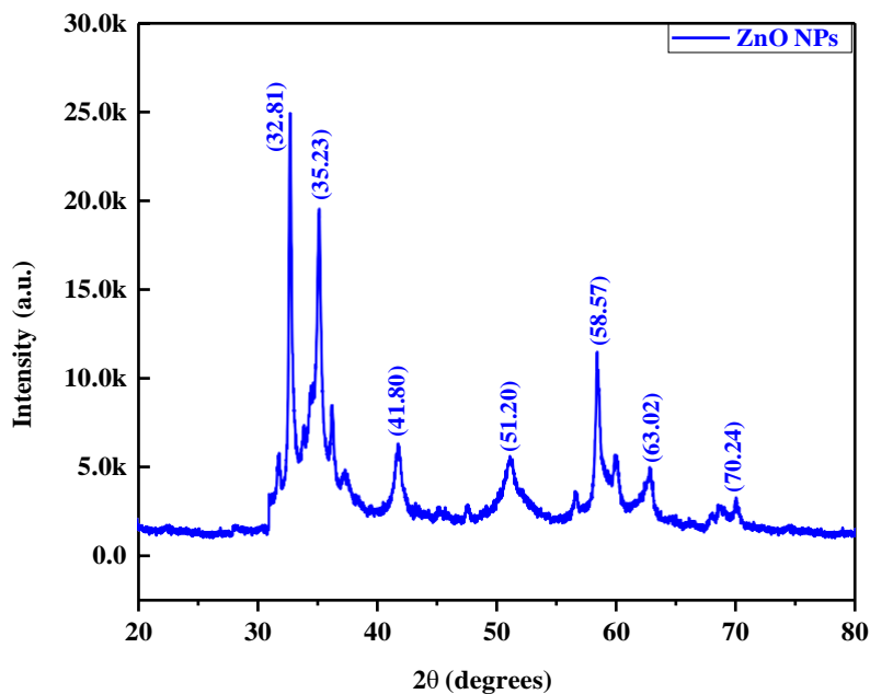
Figure 1: XRD analysis of ZnO NPs
