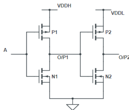
Figure 1: Basic Level Converters
