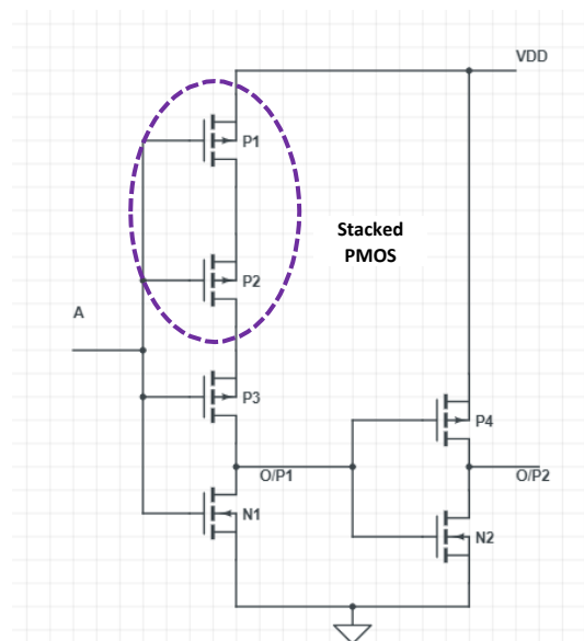
Figure 4: PMOS-based Voltage Level Converter
