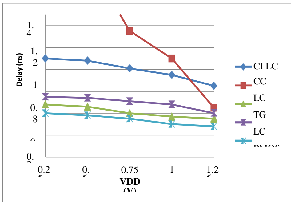
Figure 6: Simulated result analysis of Propagation delay of Level Converters as a function of VDD
