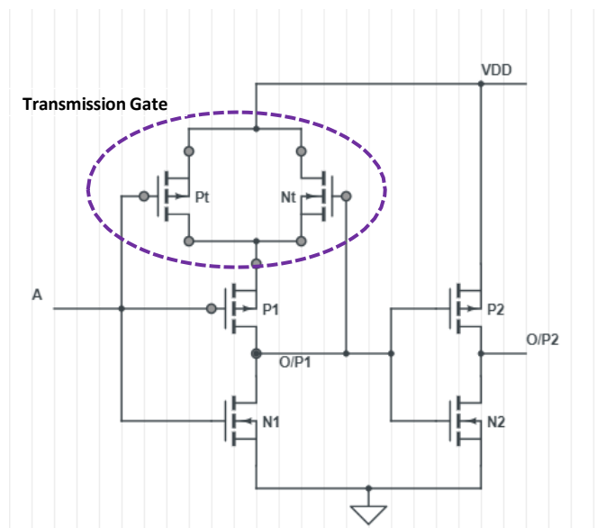
Figure 3: Transmission Gate based Voltage Level Converter
