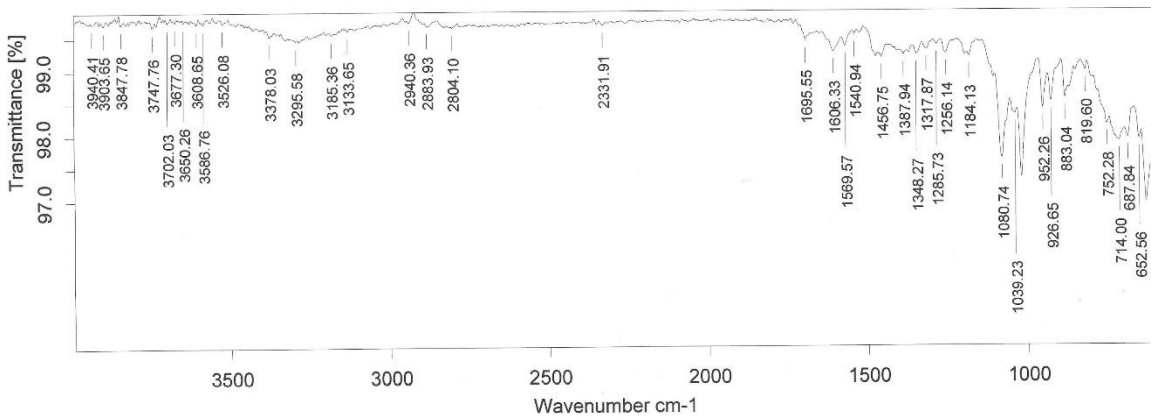
Figure 2: FTIR Spectrum of Ganciclovir + HPMC K 15
