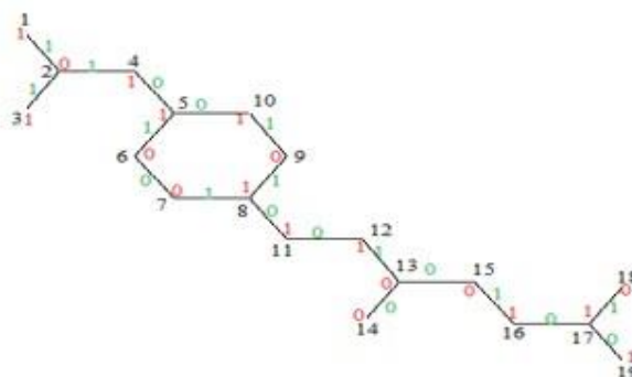
(b) Cordial-label of Atenolol
