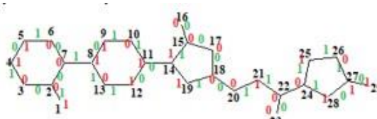
(b) Cordial-label of Rivaroxaban
