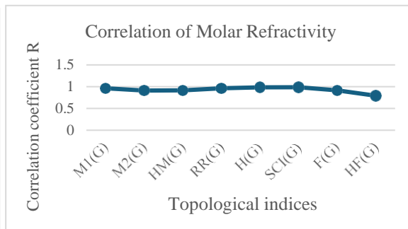
(d) Correlation between Topological indices and Molar Refractivity
