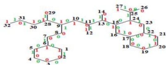
(b) Cordial-label of Quinapril
