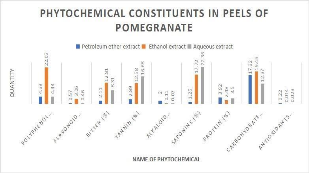
Figure 1: Graph showing comparative quantitative estimation of Phytochemical constituents in various extracts of Pomegranate peel
