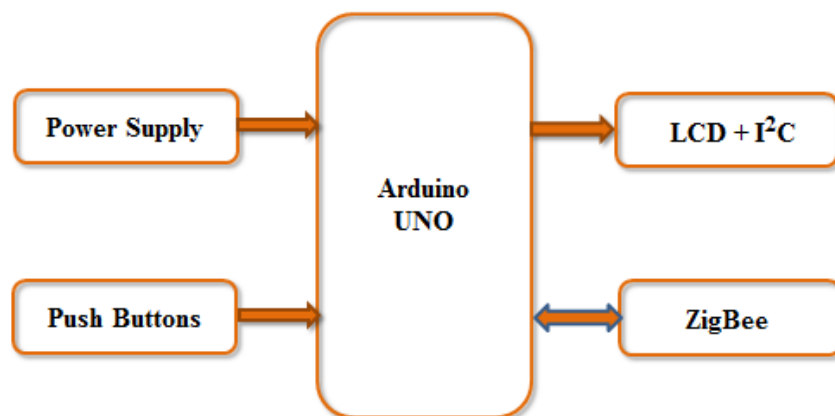
Figure 1: Block diagram of Transmitter section
