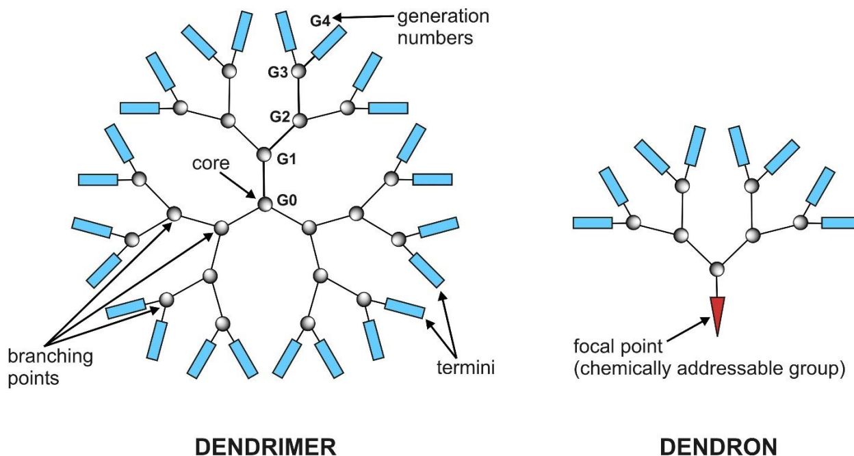
Figure 8: Dendrimers
