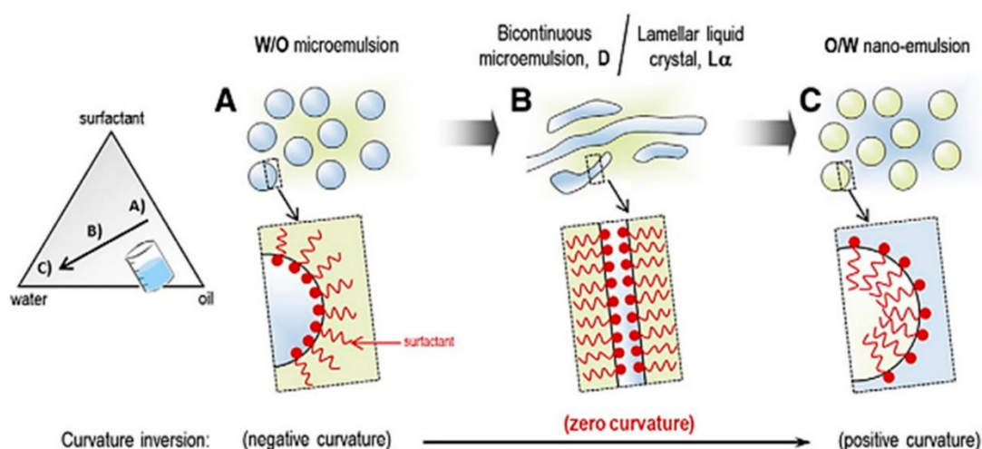
Figure 9: Nanoemulsions (NEs)
