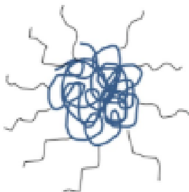
Polymeric NPs
