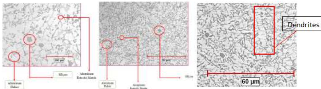
Fig.3. MICROSTRUCTURE OF SAMPLES OF THE DIE AND CORE MOLDS
