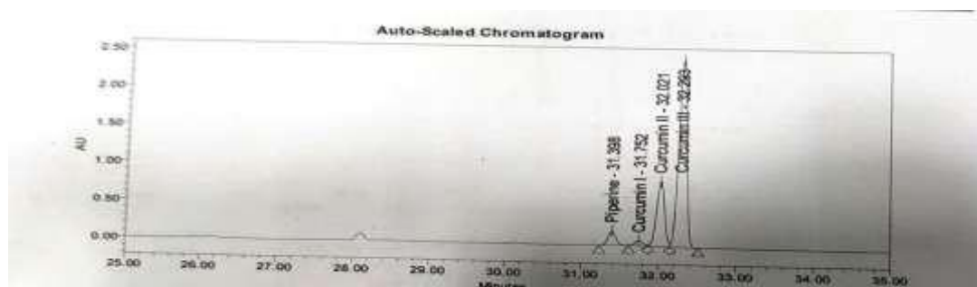
Figure 2: Typical standard chromatogram extracted at 370 nm for Piperine, Curcumin- I, Curcumin -II, Curcumin- III
