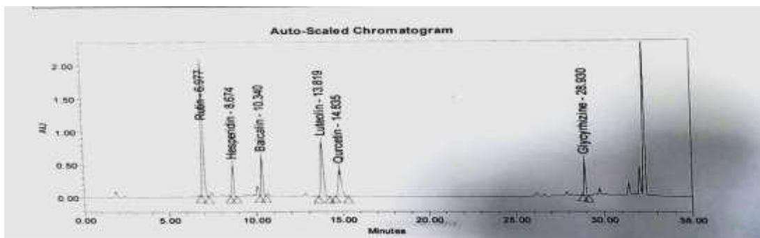
Figure 1: Typical standard chromatogram extracted at 260 nm for Rutin, Hesperidin, Baicalin, Luteolin, Quercetin and Glycyrrhizin)
