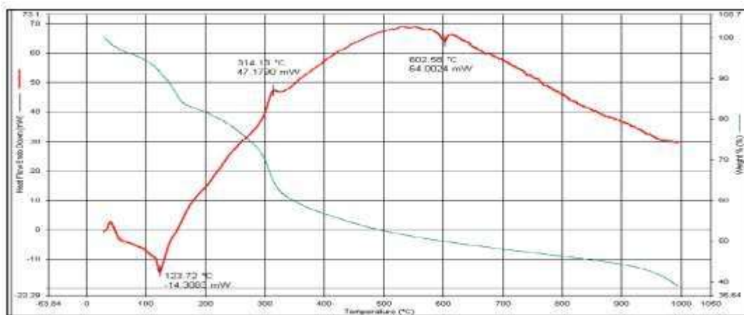
Fig 6 : DSC of Capecitabine with the excipient blend.
