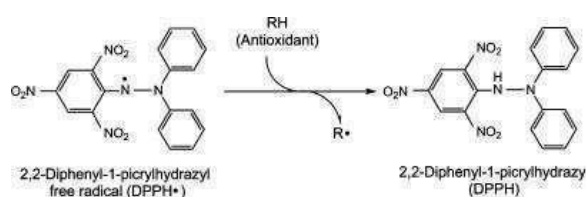
Fig-4 DPPH Mechanism of reaction
