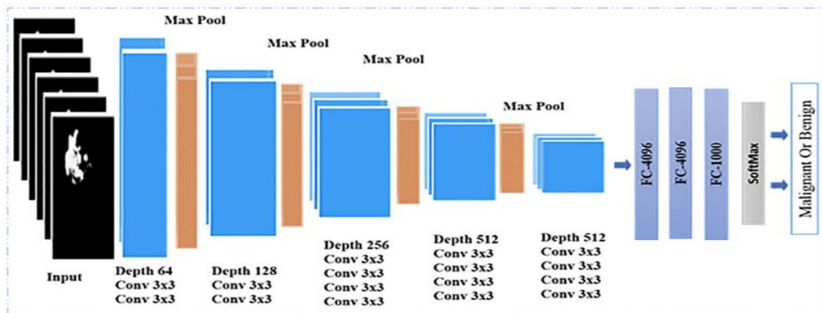
Fig 8: The suggested adjustment CNN model VGG19 for classifying brain tumors [7]
