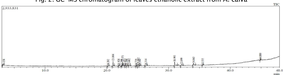
Fig. 2. GC–MS chromatogram of leaves ethanolic extract from A. calva
