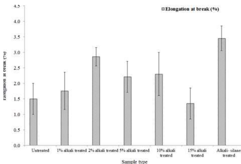
Figure 2(b): Elongation at break of untreated and treated fibers
