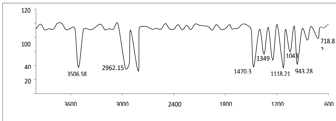
Figure 4 FTIR spectra of Stearic acid
