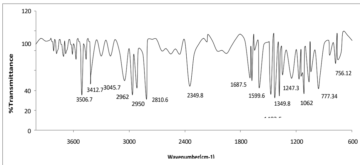
Figure 6 FTIR spectra of drug and excipient mixture
