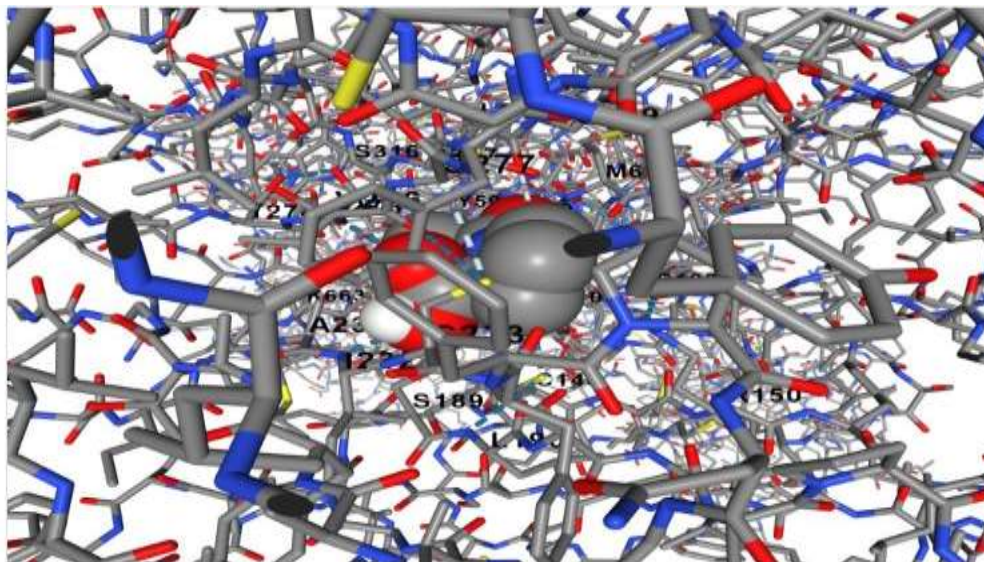
Figure 8: Molecular docking analysis in protein-ligand interaction with docking score of -5.6 MOLECULAR DOCKING BY WEB SERVER CB-Dock (mexiletine)
